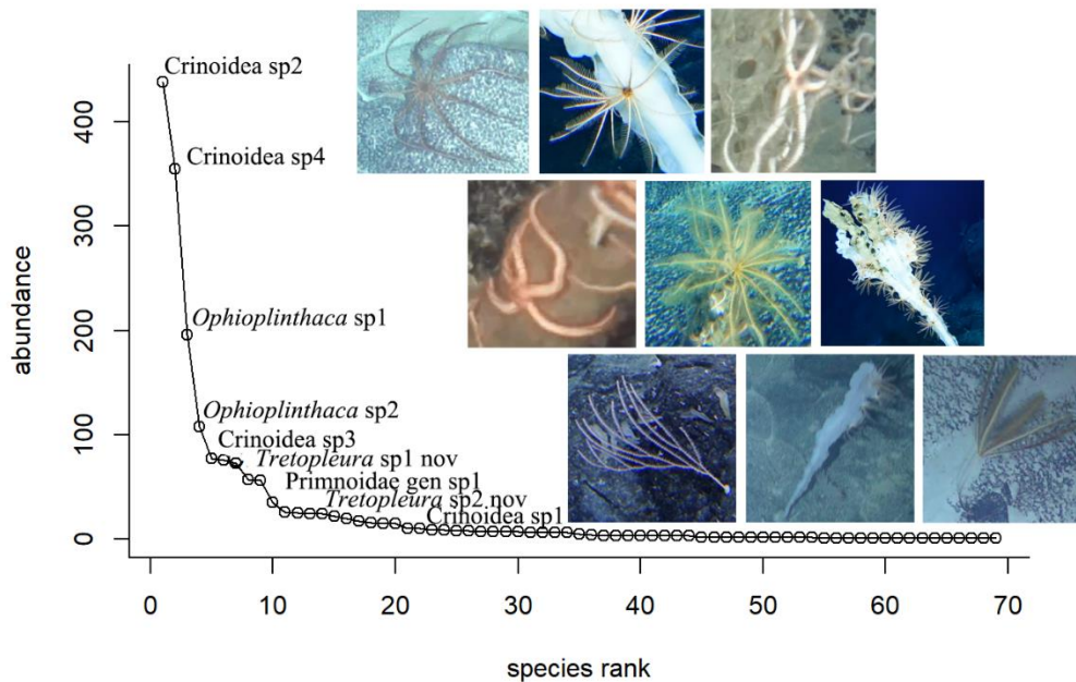
Figure 8.22 Rank-abundance curve of megafaunal morpho-species recorded from ROV dives on Weijia Guyot. Credit Cheng-Cheng Shen and Dong-Sheng Zhang.
