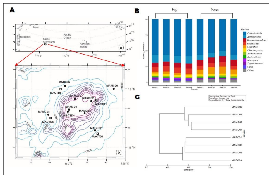
Figure 8.4 A: Location of Caiwei Seamount and sampling sites (stations at the seamount top: MAMC01-MAMC04; stations at the seamount base: MABC02, MAMC08, MAMC06, MABC06); B: bacterial composition at the top and base of the seamount; C: microbial clustering analysis in sediments from the top and base of the seamount. Modified from Liu et al. (2019).
