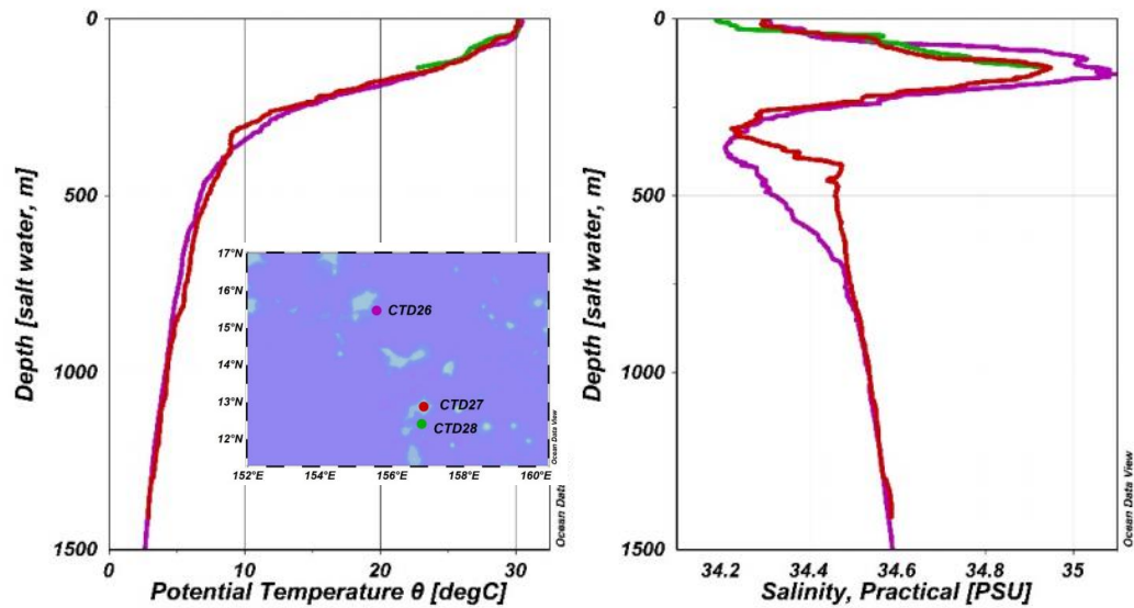
Figure 6.6 Typical vertical profile of temperature (left) and salinity (right) near Caiwei Seamount obtained by CTD (COMRA DY56 cruise report). Credit Jun Wang.
