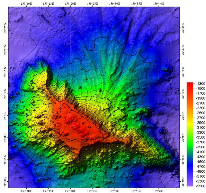
Figure 4.13 Topographic map of Suda Seamount. Data from China Ocean Voyage Survey (unpublished data). Credit Huaiming Li and Zhenggang Li
