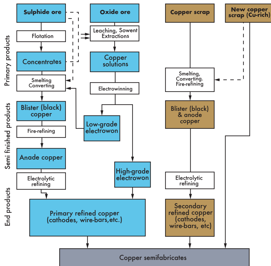
Figure 4.3. Copper value chain
