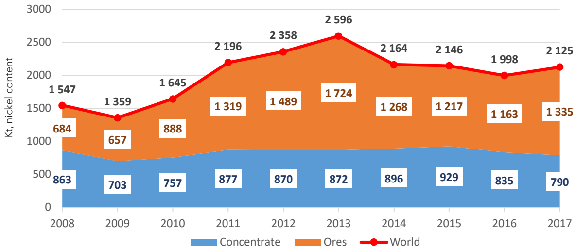
Figure 4.51. World nickel mine production by type in 2008-2017
