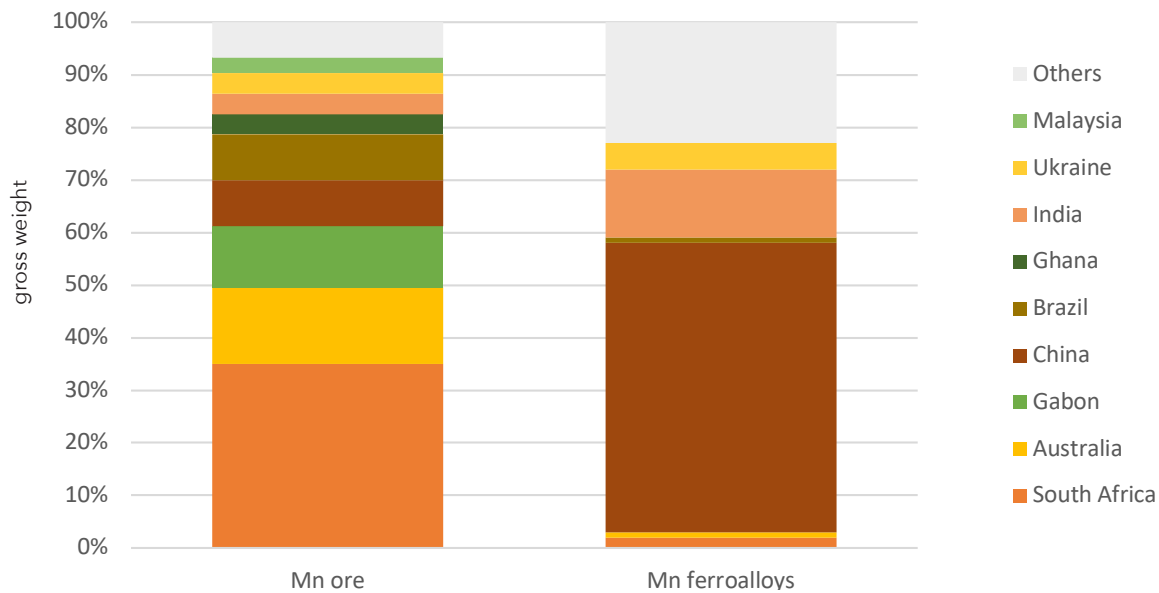
Figure 4.62. Distribution of production of manganese ore by content of manganese and ferro-alloys among major countries in 2017
